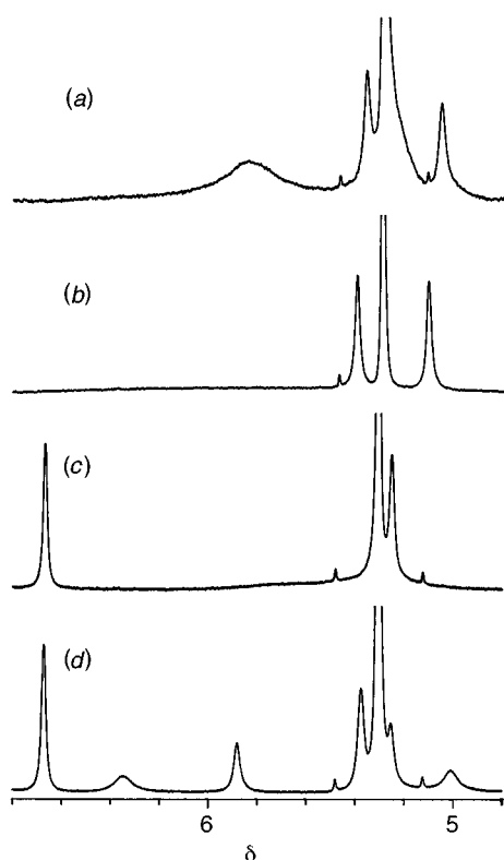
Fig. 8 The ^1\text{H} NMR spectra of [\text{HgPh}(\text{tftsc})] 7 in \text{CD}_2\text{Cl}_2 at (a) 297, (b) 277, (c) 220 and (d) 193 K (spectra contain additional solvent peaks)
