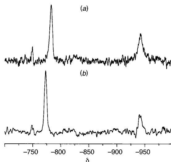
Fig. 7 The 199 Hg NMR spectra (297 K) of (a) [HgPh(btsc)] 3 and (b) [HgPh(mbts)] 5
